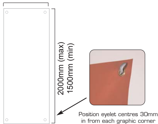
Graphic dimensions and eyelet positioning
